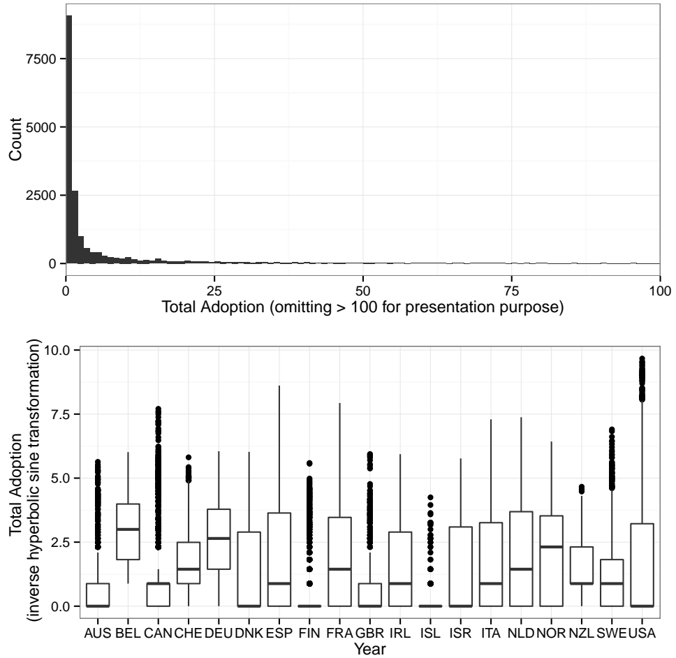
FIG B.2. Excess Zeros and Clustering in Directed Dyad Adoption Data. The top panel shows that 9064 out of 19112 directed dyad-years (or 47.43%) have zero adoptions. Furthermore, 77.98% of all non-zero adoption directed dyad-years have between 1 and 30 adoptions (approximately the mean). The boxplot in the bottom panel shows that dyadic adoption counts further cluster by receiving country. Inverse hyperbolic sine transformation was done for total adoption counts to give clearer picture of clustering.
