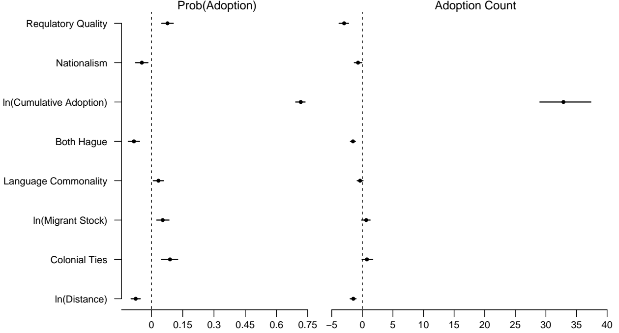
FIG 6. Substantive Effects of Key Covariates on the Predicted Probabilities and Expected Counts of International Adoption. Substantive effects are simulated based on first differences, i.e. calculated as the change in the expected value (probability or count) when the covariate of interest is changed from zero to one for a dichotomous independent variable, or increased from one standard deviation under the mean to one standard deviation above the mean for a continuous covariate, while holding all other covariates at their mean or mode and setting the receiving country to USA and the year to 2000.
